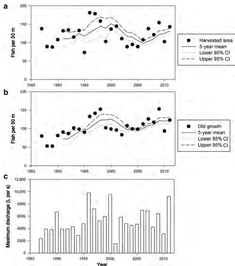
Figure 5. Temporal trends of trout abundance in (a) harvested and (b) old-growth forest with 5-year running means and (c) maximum discharge in streams in the H. J. Andrews Experimental Forest, in Oregon. Contrary to expectations of decreased fish density after a flood, a 35–50-year flood in 1996 resulted in increases of cutthroat trout densities in both the old-growth reference reach and the downstream reach through young forests. Abbreviations: L, liters; m, meters; s, seconds.
